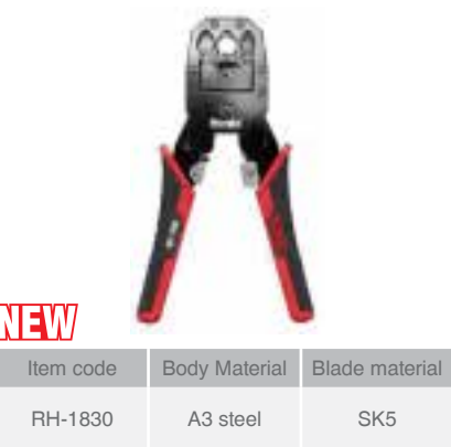
Modular Plug Crimper
